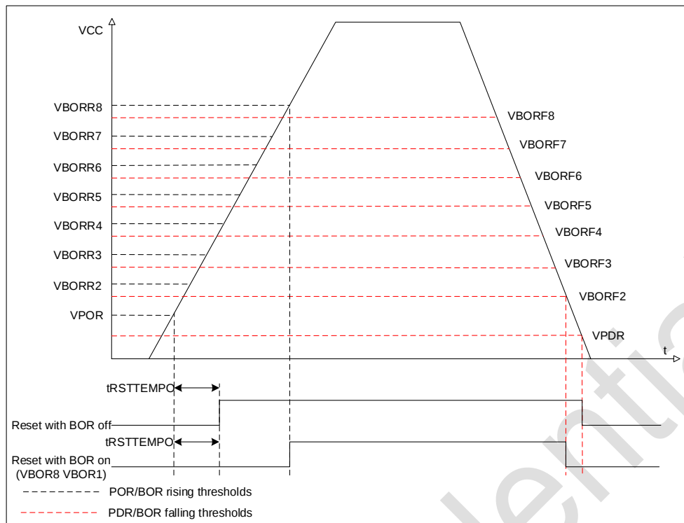
Figure 2-3 POR/PDR/BOR threshold
